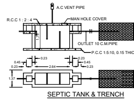
SEPTIC TANK & TRENCH
