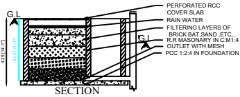
RAIN WATER HARVESTING OF RECHARGE TRENCH METHOD
