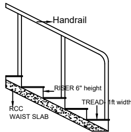
Staircase Detail
