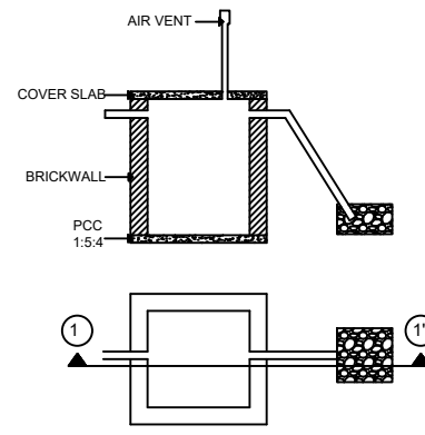
Septic Tank
