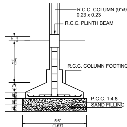
Footing Detail
