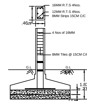
RCC COLUMN DETAILS
