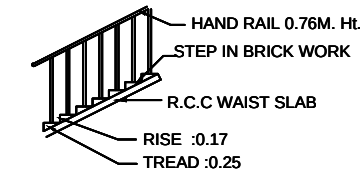
STAIR CASE DETAIL
