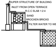
RAINWATER HARVESTING
