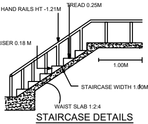
STAIRCASE DETAILS
