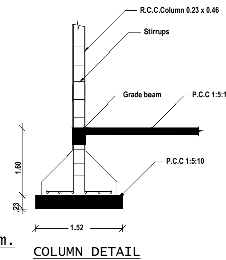
COLUMN DETAIL
