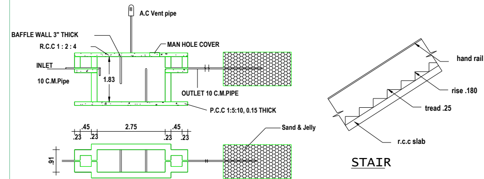
SEPTIC TANK AND TRENCH
