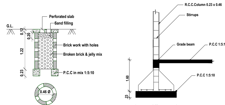
PERCOLATION PIT FOR 30 Sq. m. (Scale:- 1:50)
