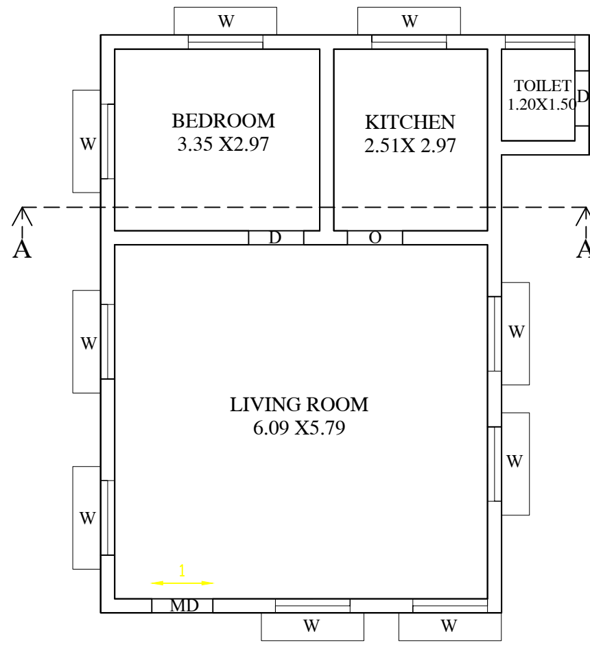
ED GROUND FLOOR PLAN
