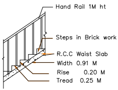
STAIRCASE DETAILS
