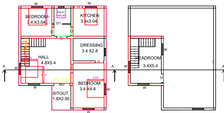
G.F. PLAN
