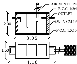
SEPTIC TANK & TRENCH
