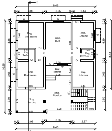
EXG. GROUND FLOOR PLAN
