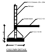
COLUMN DETAIL
