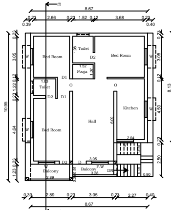
PRO. FIRST FLOOR PLAN
