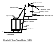
Detail of Solar Water Heater (SWH)
