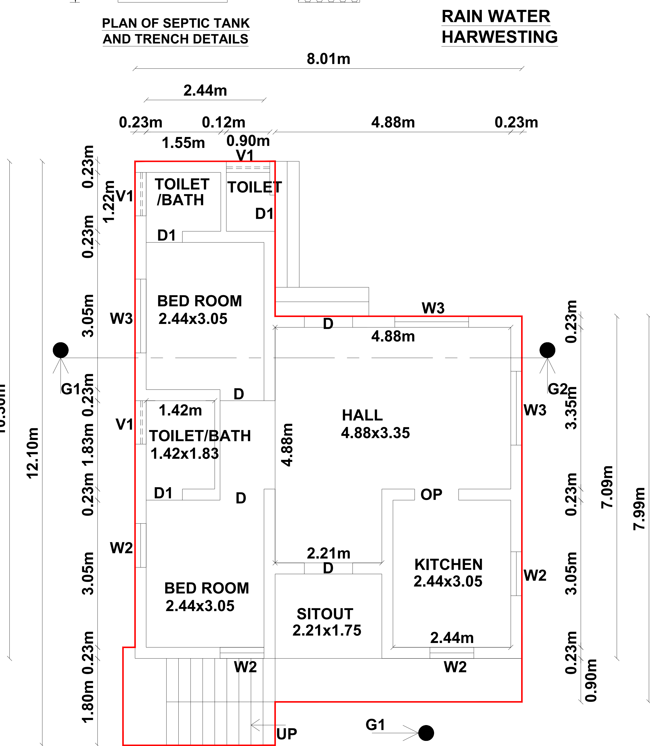
PLAN (Proposed)
