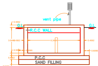
SECTION ON D-D
