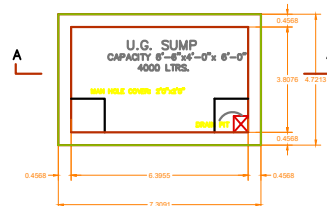
SUMP DETAIL
