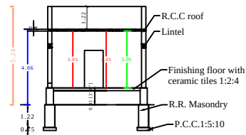
SECTION AB
