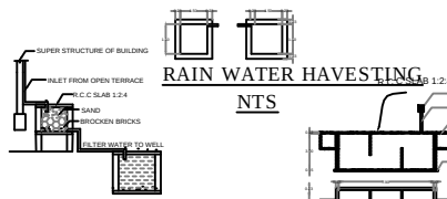
DETAILS OF FILTER BED & WELL
