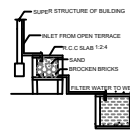
DETAILS OF FILTER BED & WELL NTS
