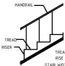
STAIRCASE DETAILS NTS
