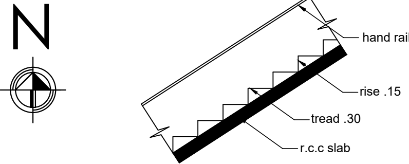
STAIR
