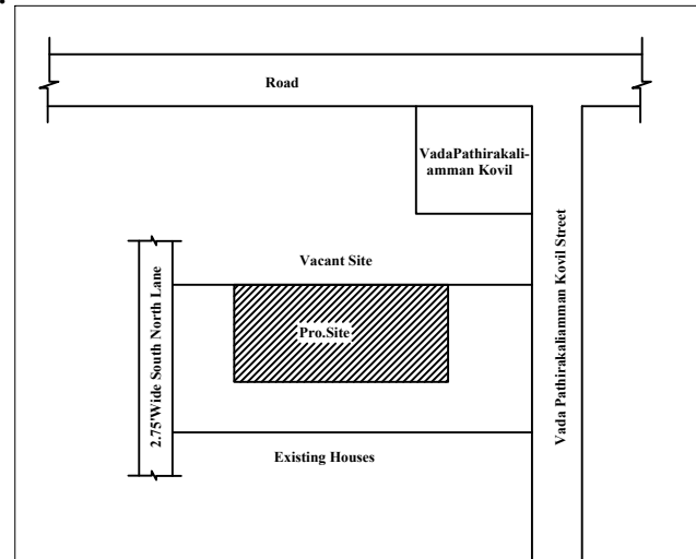
LOCATION PLAN
