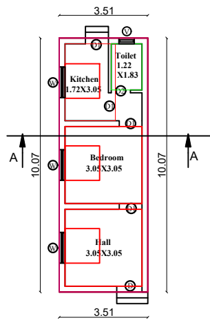
PLAN
