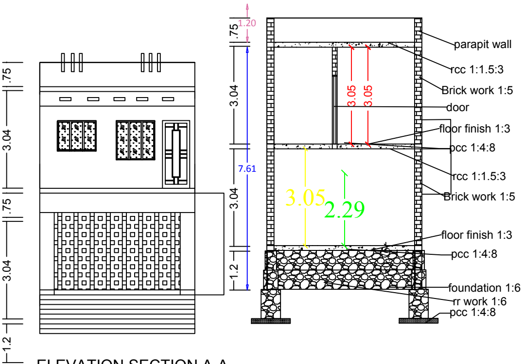
ELEVATION SECTION A-A
