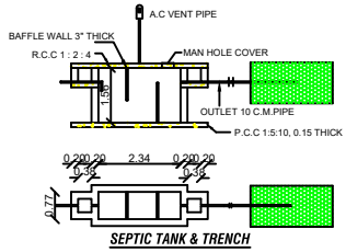
SEPTIC TANK & TRENCH
