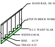
STAIR DETAIL
