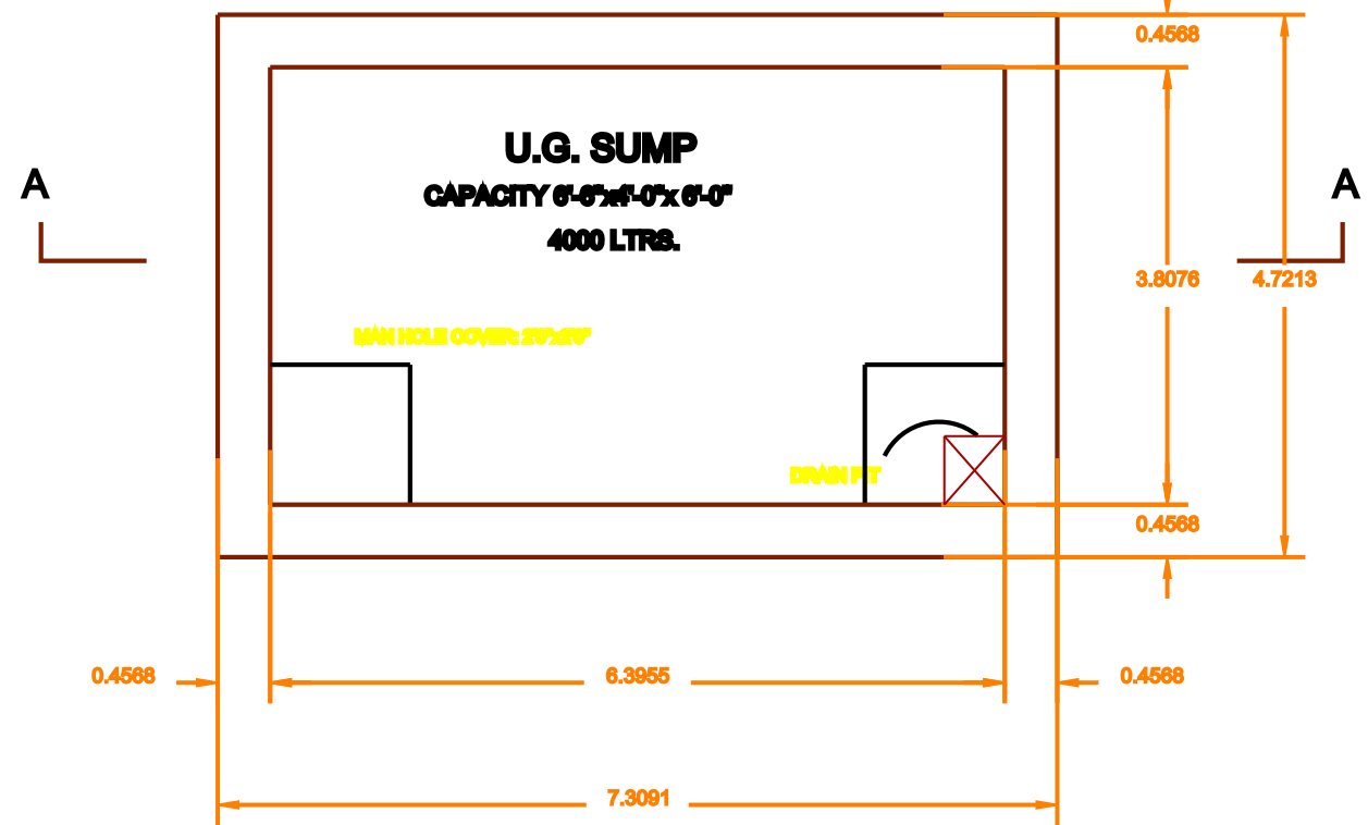
SUMP DETAIL
