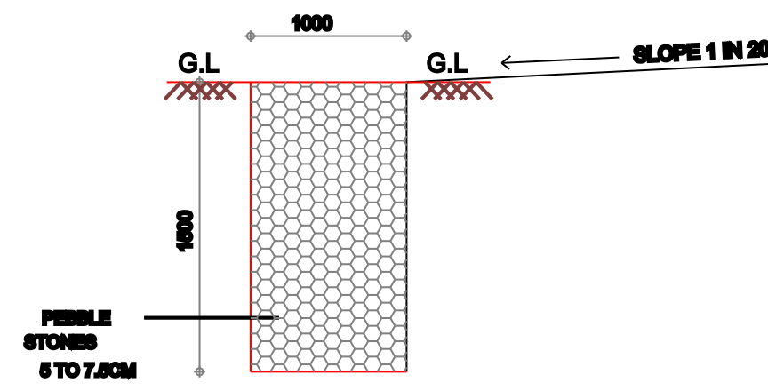
SECTION OF PEBBLE TRENCH
