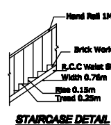
STAIRCASE DETAIL
