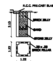
PLAN & SECTION OF RAIN WATER COLLECTION WELL
