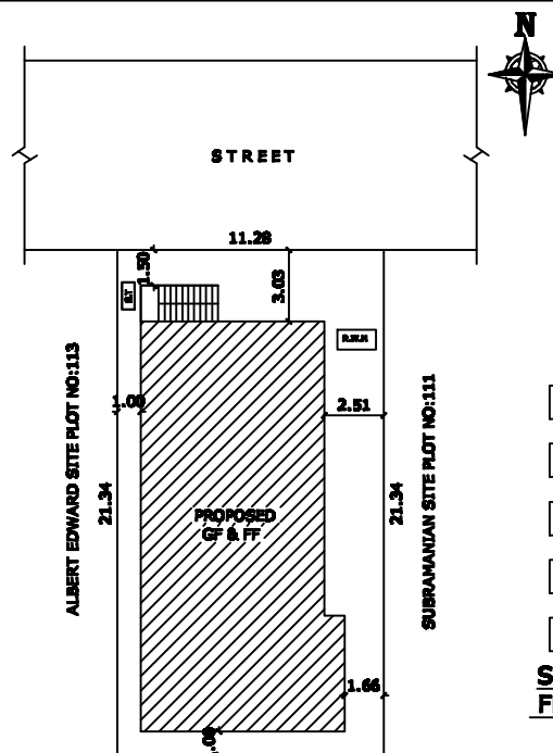
SITE PLAN
