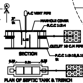
SECTION PLAN OF SEPTIC TANK & TRENCH
