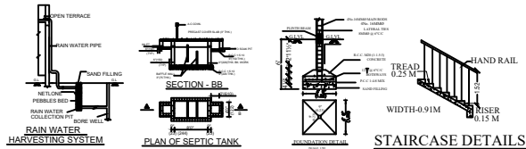
RAIN WATER HARVESTING SYSTEM
