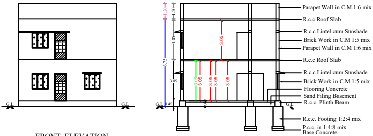
FRONT ELEVATION
