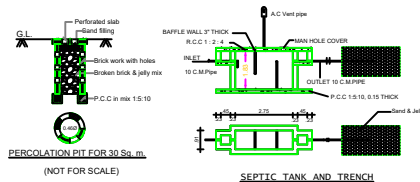
SEPTIC TANK AND TRENCH
