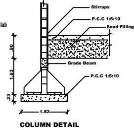
COLUMN DETAIL
