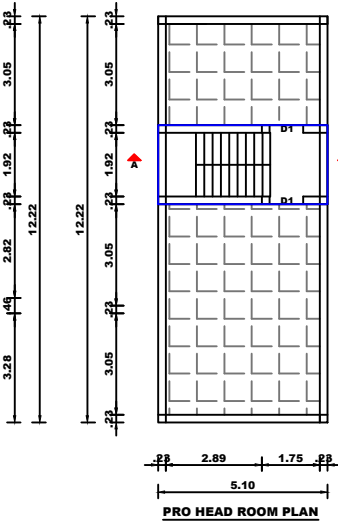
PRO HEAD ROOM PLAN
