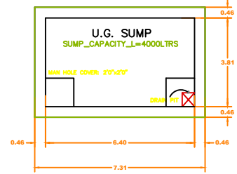
SUMP DETAIL
