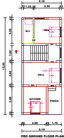
PRO GROUND FLOOR PLAN
