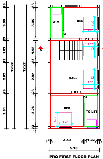
PRO FIRST FLOOR PLAN
