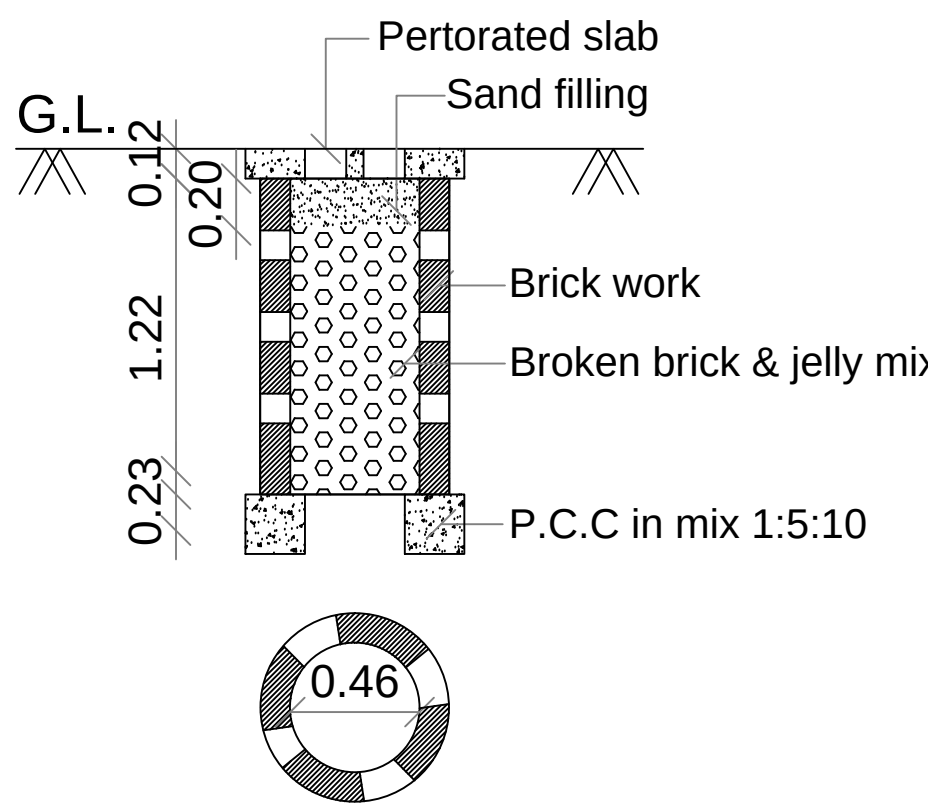
PERCOLATION PIT
