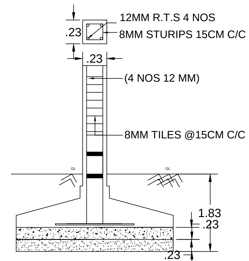
RCC COLUMN DETAILS
