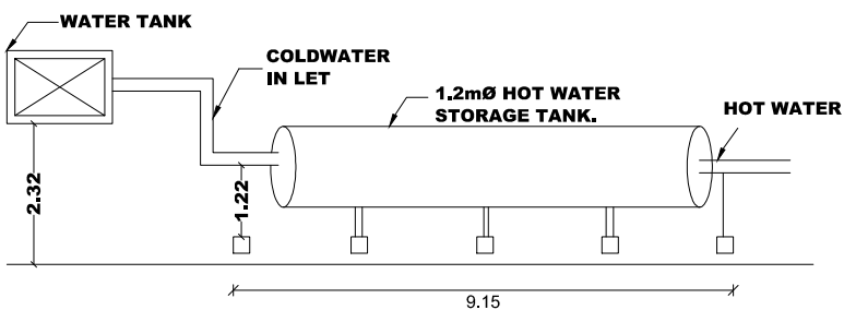
SOLAR WATER HEATING SWHS DETAIL
