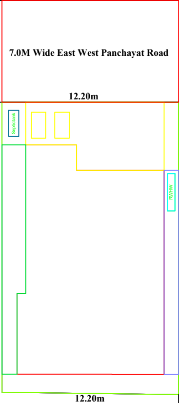
SITE PLAN
