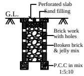
PERCOLATION PIT (NOT FOR SCALE)
