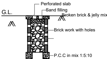
RAINWATER HARVESTING
