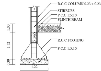
COLUMN DETAILS
