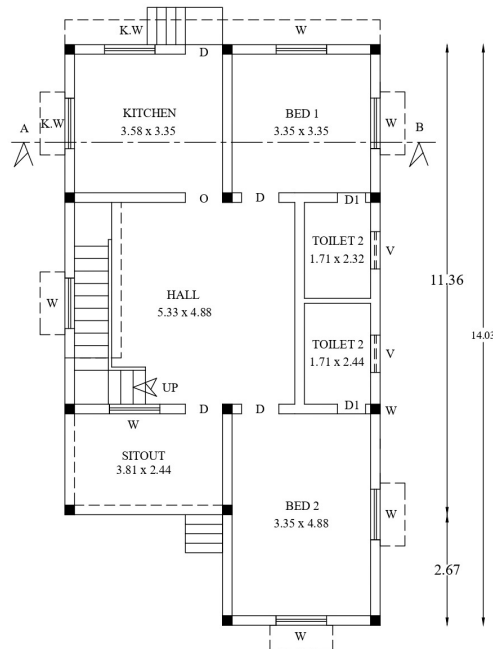
PLAN
