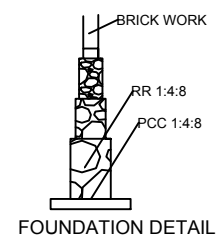
FOUNDATION DETAIL
