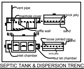
SEPTIC TANK & DISPERSION TRENCH
