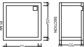
DETAILS OF COLLECTION TANK FOR RAIN WATER HARVESTING OF ROOF TOP RAIN WATER
