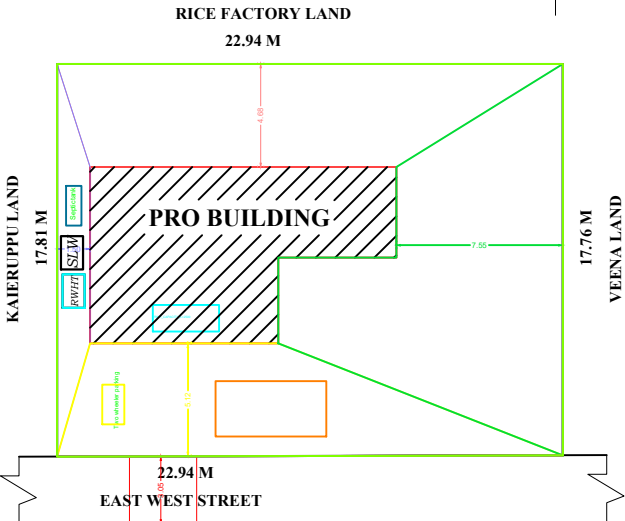
SITE PLAN
