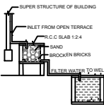
DETAILS OF FILTER BED & WELL NTS
