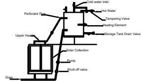
Details of Solar Water Heater (NTS)
