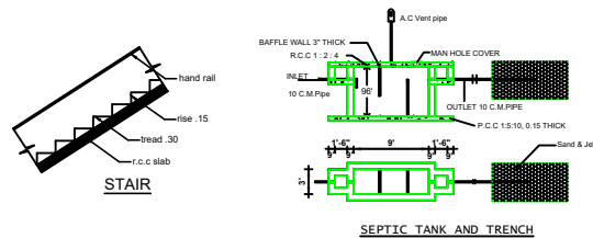
SEPTIC TANK AND TRENCH
