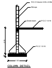
COLUMN DETAIL
