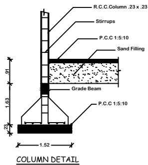
COLUMN DETAIL
