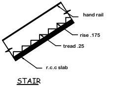
STAIR
