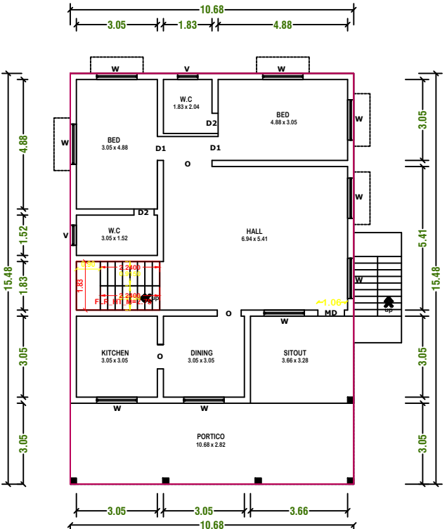
EX.GROUND FLOOR PLAN
