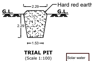
Scale 1:100
