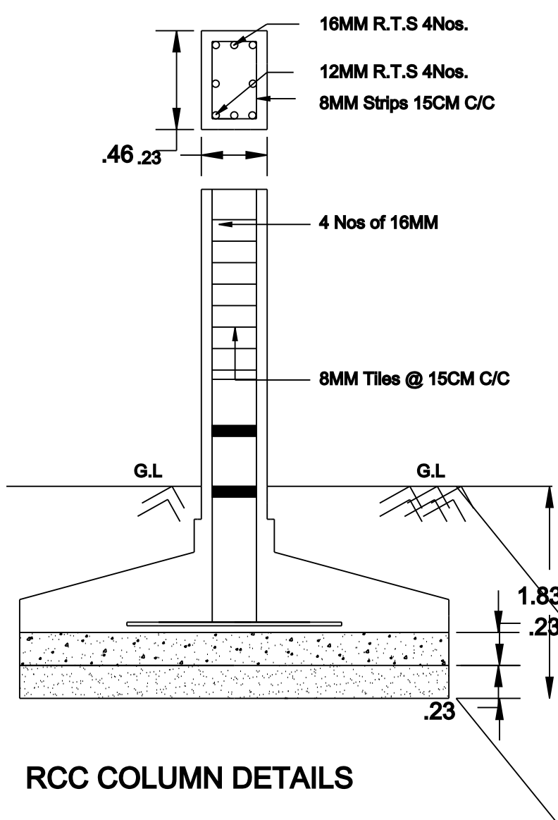
RCC COLUMN DETAILS
