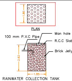
RAINWATER COLLECTION TANK
