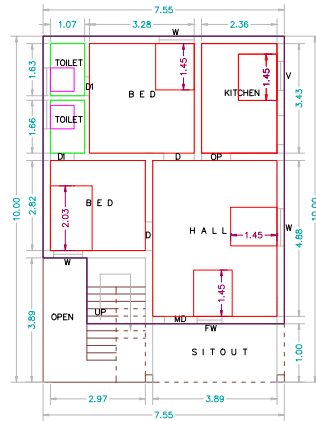
PRO.G.FLOOR PLAN SCALE 1:100
