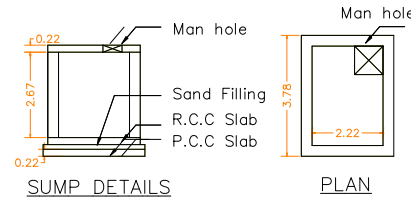
SUMP DETAILS
