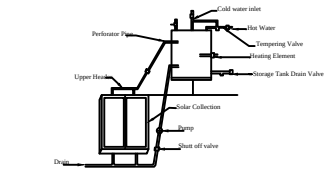
Details Of Solar Water Heater (NTS)
