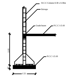
Column Detail
