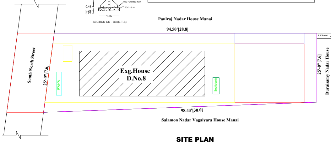
SITE PLAN
