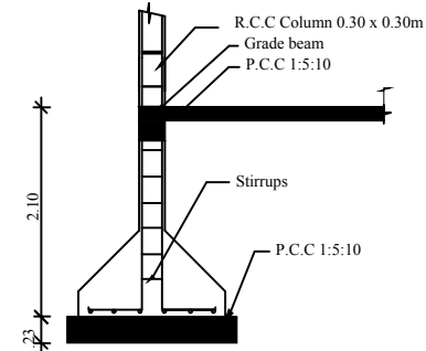
Column Detail
