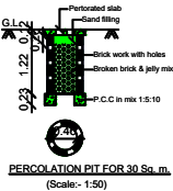
PERCOLATION PIT FOR 30 Sq. m. (Scale:- 1:50)
