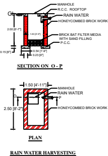
RAIN WATER HARVESTING
