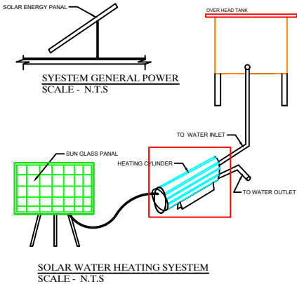
SOLAR WATER HEATING SYSTEM SCALE - N.T.S
