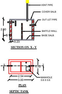
SEPTIC TANK
