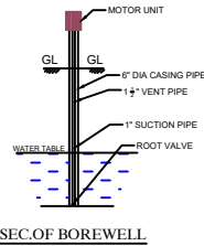
SEC.OF BOREWELL
