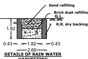
DETAILS OF RAIN WATER HARVESTING
