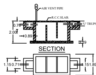
SEPTIC TANK PLAN
