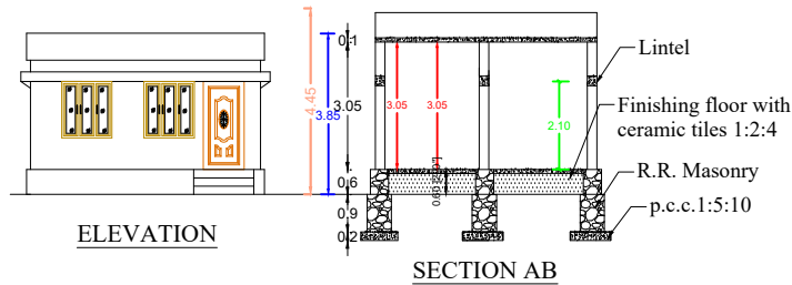
SECTION AB
