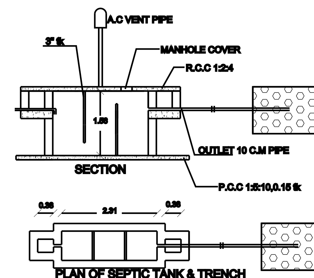
PLAN OF SEPTIC TANK & TRENCH
