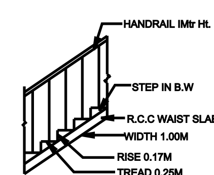
STAIR DETAIL
