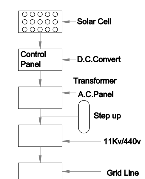
SOLAR SYSTEM FLOW DIAGRAM
