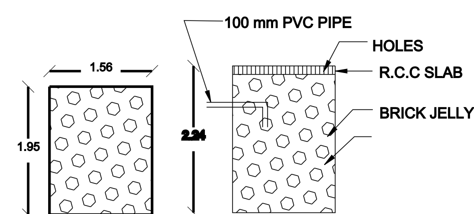
PLAN & SECTION OF RAINWATER COLLECTION TANK
