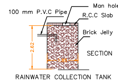
RAINWATER COLLECTION TANK
