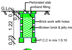
PERCOLATION PIT FOR 30 Sq. m. (Scale:- 1:50)
