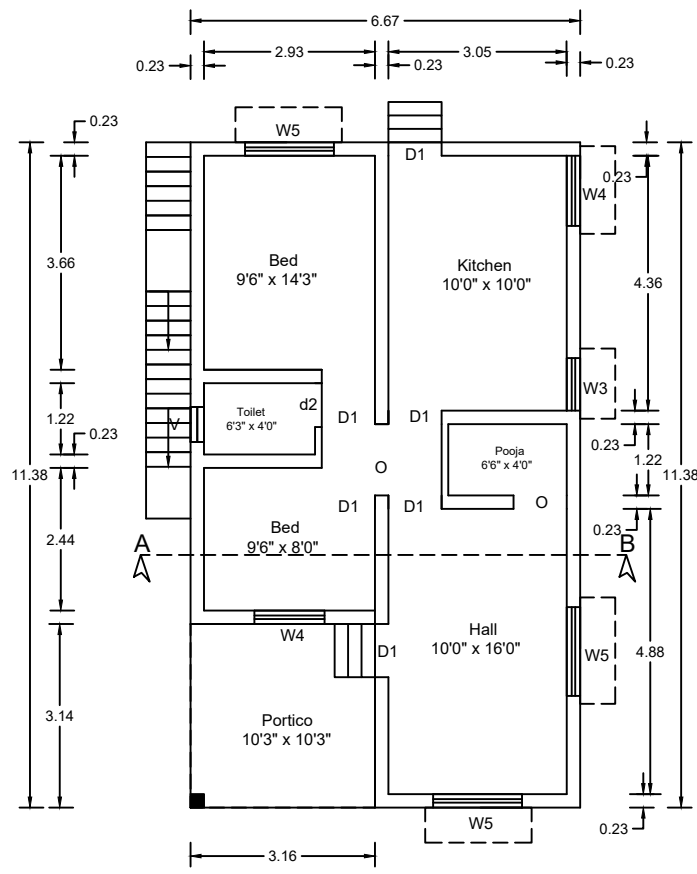
EXTG. GROUND FLOOR PLAN
