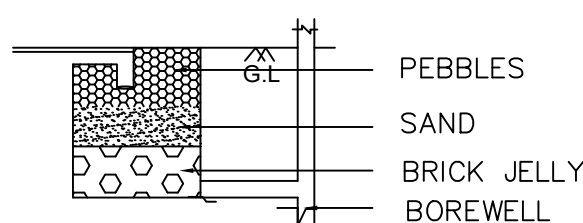
RAINWATER FILTRATION
