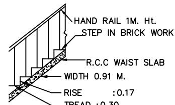
STAIR DETAIL
